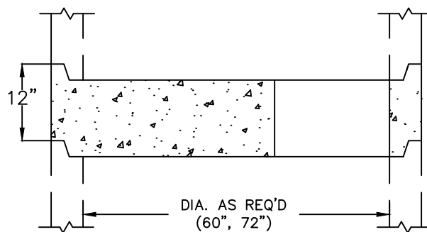
SAFETY PLATFORM DETAIL NOT TO SCALE
