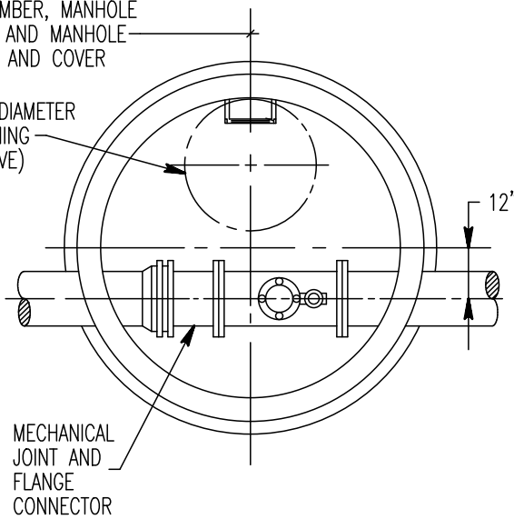
SECTIONAL PLAN
