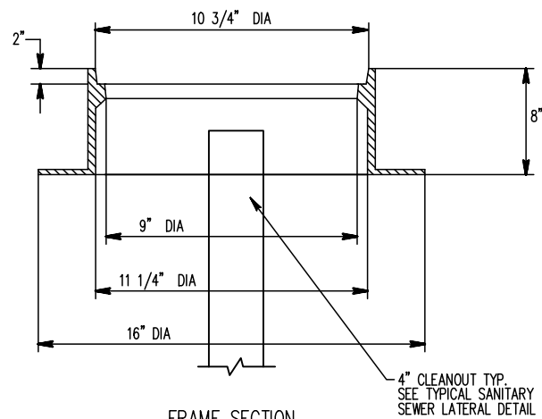
FRAME SECTION
