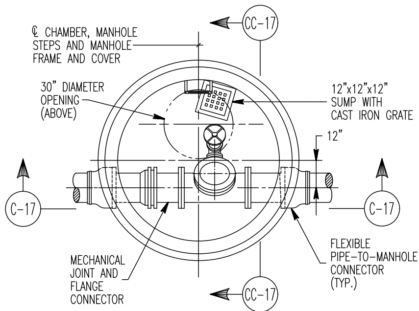
SECTIONAL PLAN
