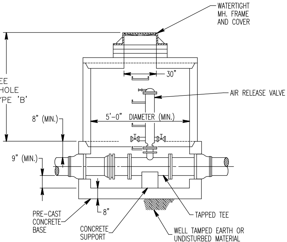
SECTIONAL ELEVATION
