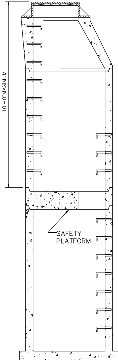
MANHOLE CROSS-SECTION NOT TO SCALE
