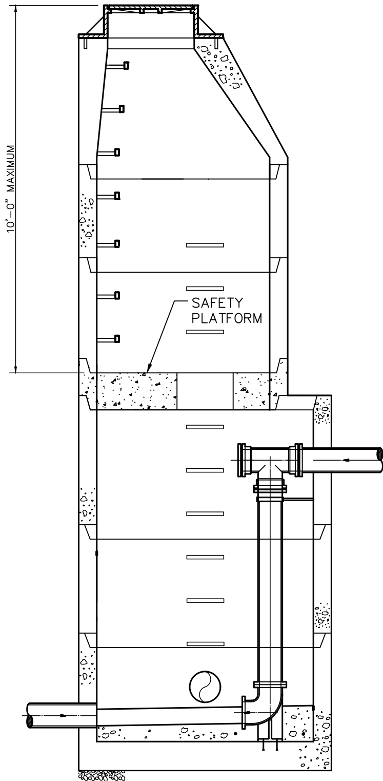
MANHOLE CROSS-SECTION NOT TO SCALE
