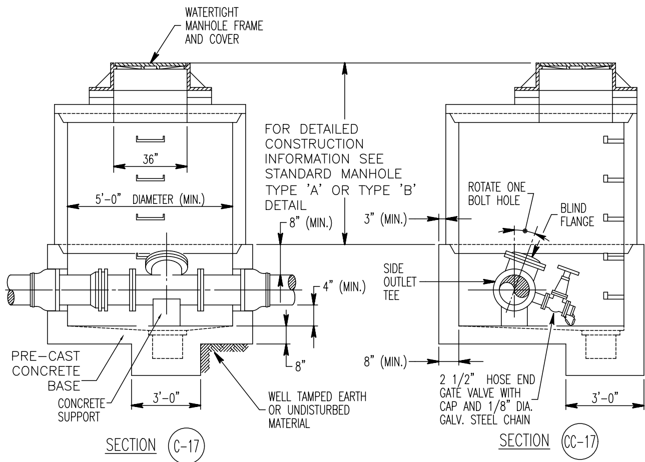
CLEANOUT CHAMBER
