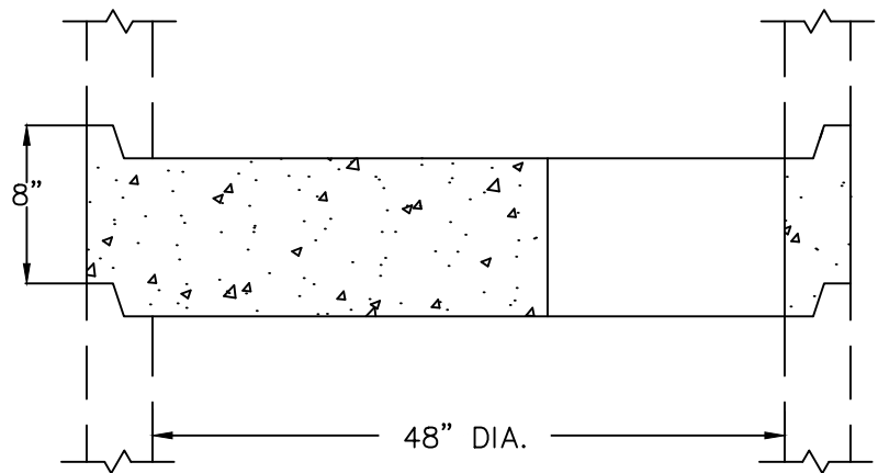
SAFETY PLATFORM DETAIL NOT TO SCALE
