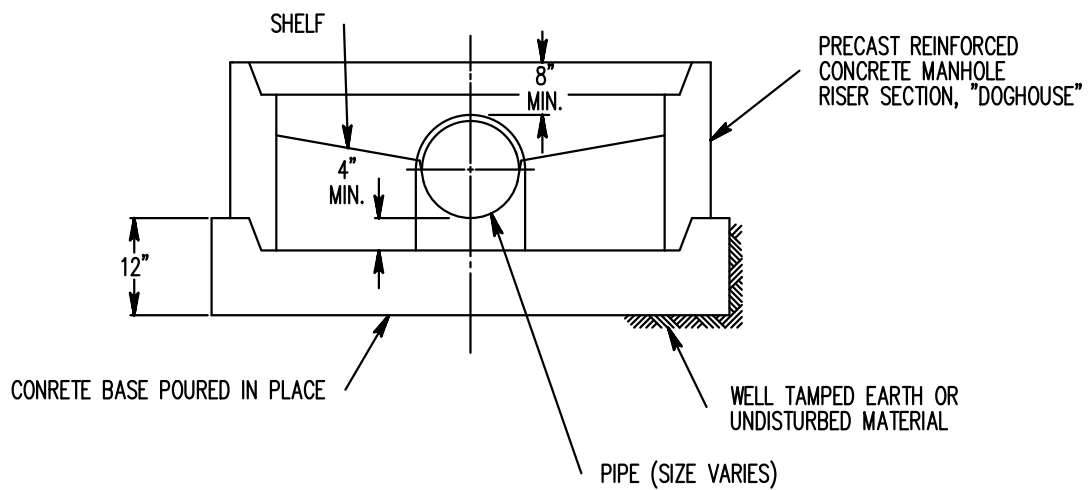
SECTIONAL ELEVATION "DOGHOUSE" MANHOLE SECTION AND BASE
