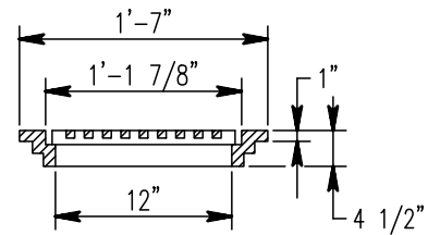
SECTIONAL ELEVATION
