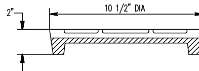
COVER SECTION
