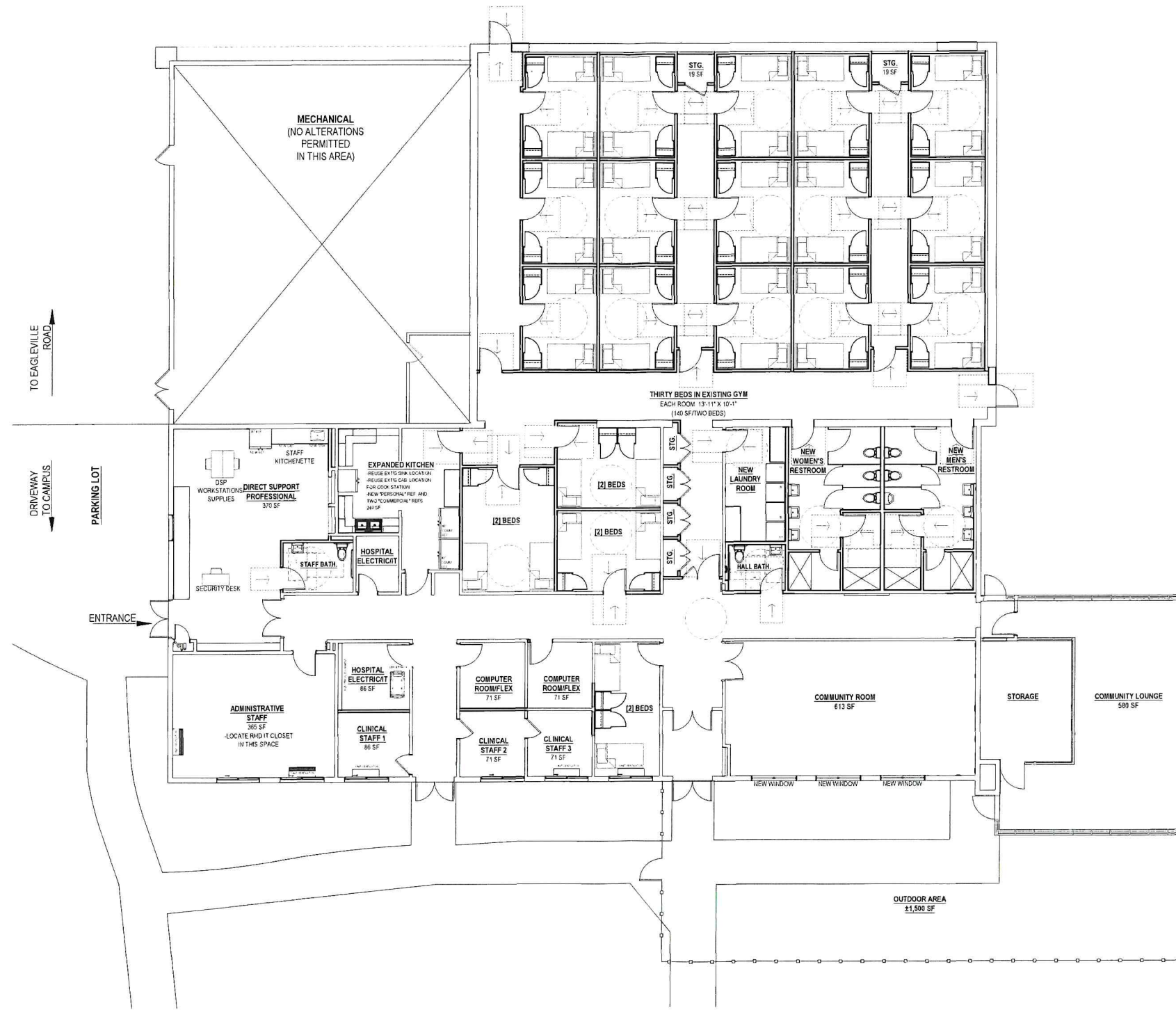
1 PRICE BUILDING - SCHEMATIC PLAN SD1.0 / 1/8" = 1'-0"
